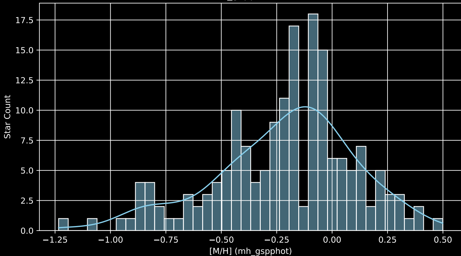
APOGEE DR17 Field: [149+62_MGA [M/H] (mh_gspphot) (n= 172)
