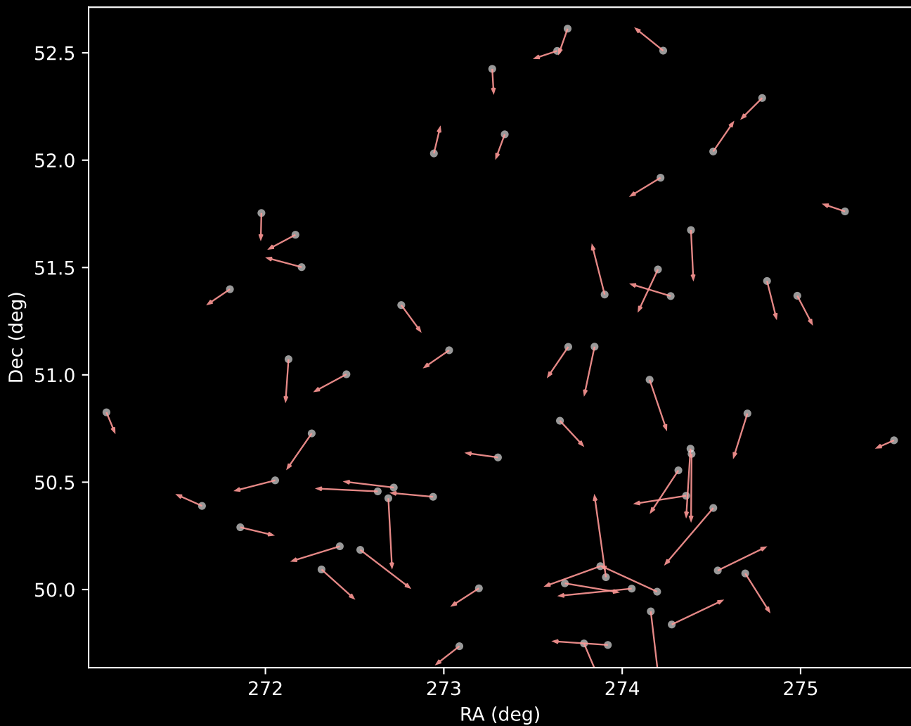
APOGEE DR17 Cluster 7 Proper Motion Vectors (n=61)
