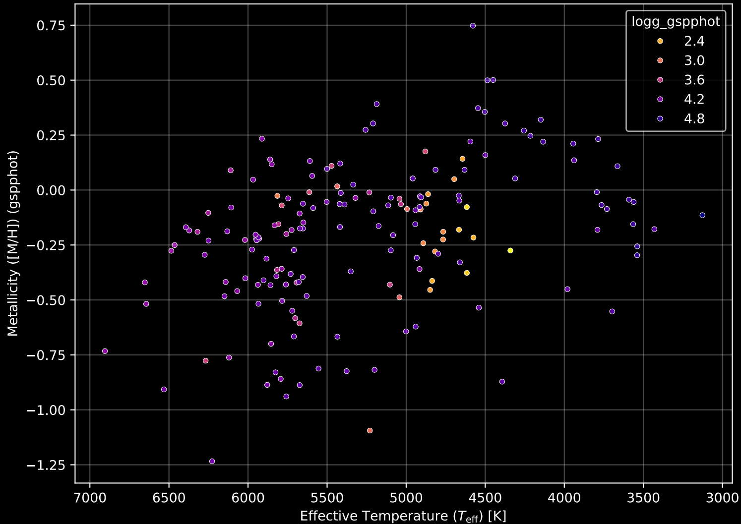
APOGEE DR17 Field: [149+62_MGA] Stellar Population Parameters (n= 174)
