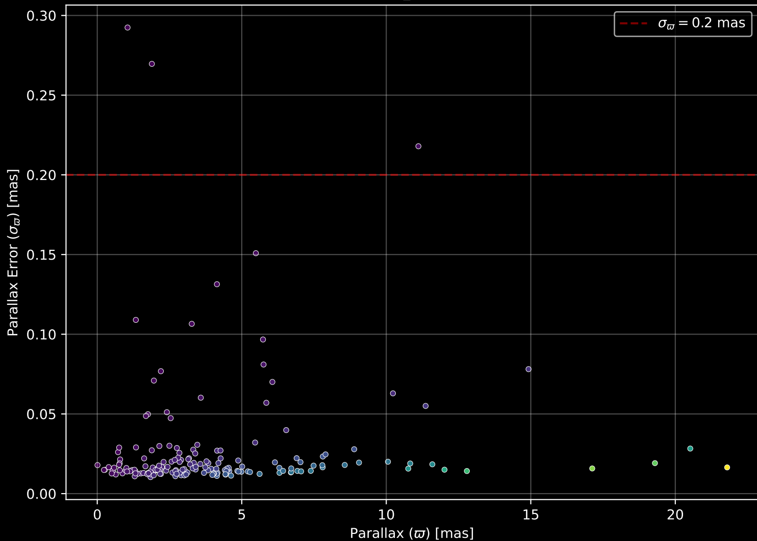
APOGEE DR17 Field: [149+62_MGA] Parallax Quality (n= 174)
