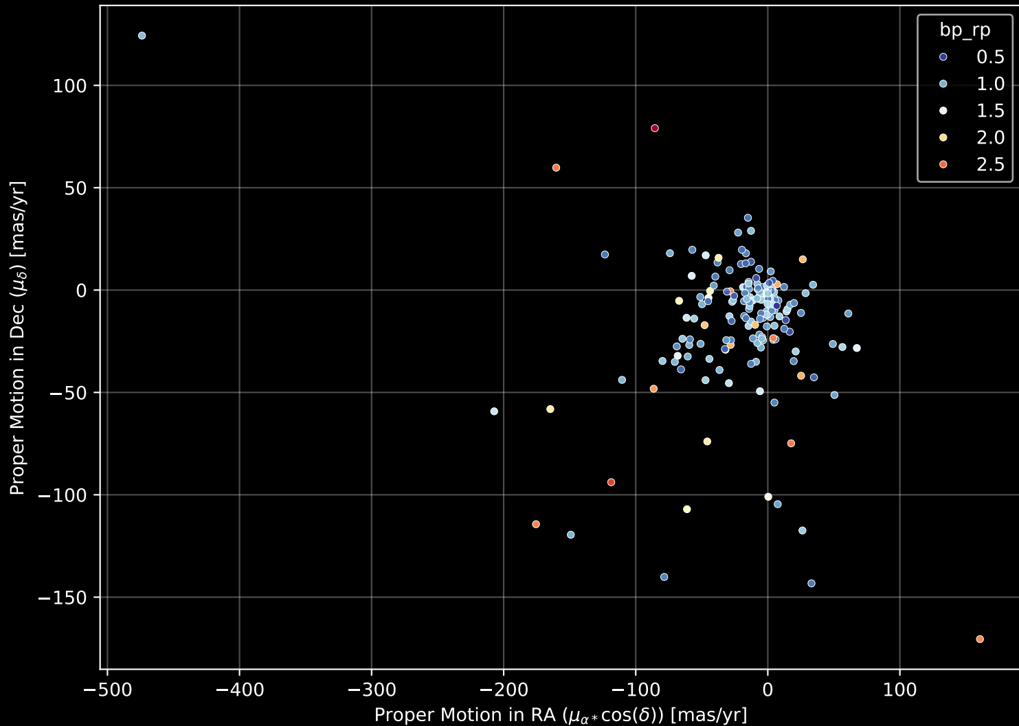
APOGEE DR17 Field: [149+62_MGA] Proper Motion Diagram (n= 174)
