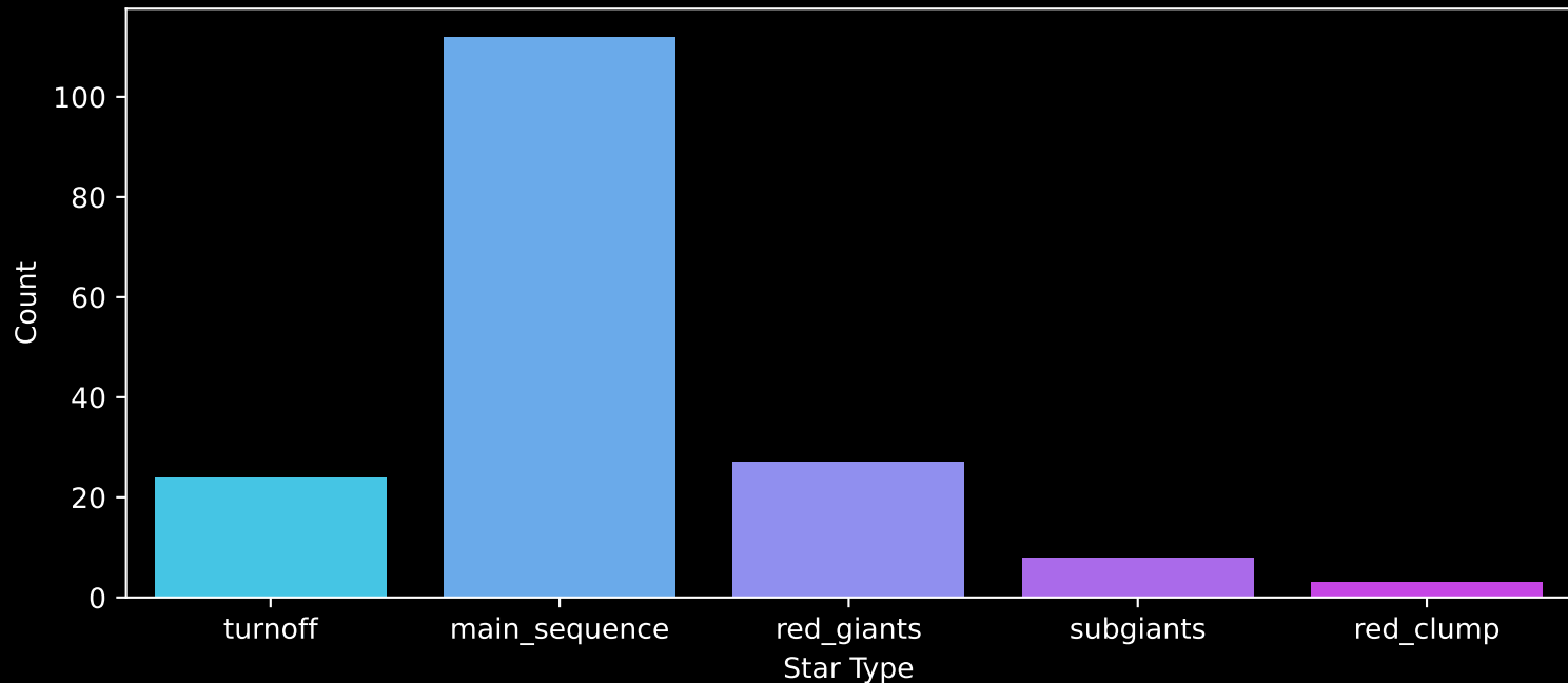
APOGEE DR17 Field: [149+62_MGA] Count plot of Star Type
